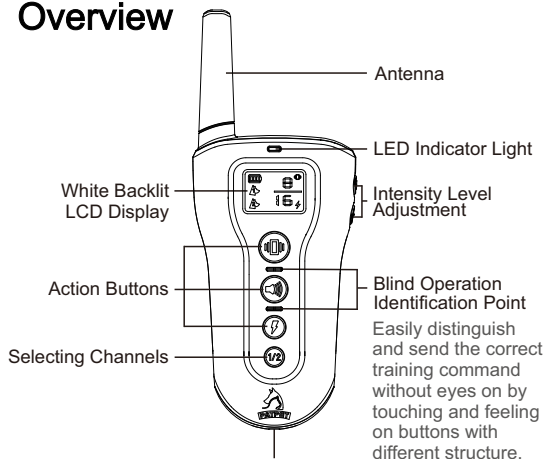
Transmitter
